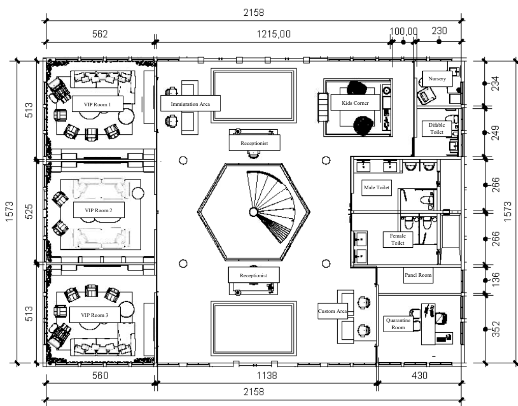
LAYOUT - LANTAI 1 GENERAL SKALA 1 : 200
